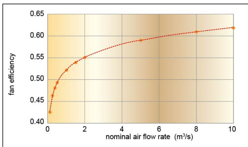
Image 1: Fan efficiency \eta_{\text{fan}} as a function of nominal air flow q_{\text{nom}}
